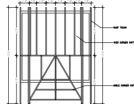
5 ROOF FRAMING SCALE: 1/4" = 1'-0"
