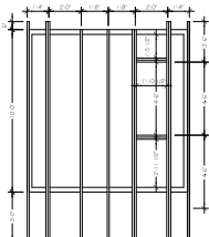
3 LOFT FLOOR FRAMING SCALE: 1/4" = 1'-0"
