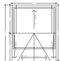
6 ROOF PLAN SCALE: 1/4" = 1'-0"
