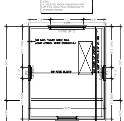
4 LOFT FLOOR PLAN SCALE: 1/4" = 1'-0"
