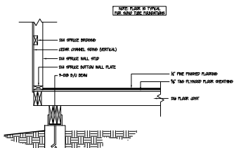
12 FLOOR DETAIL SCALE: 1" = 1'-0"
