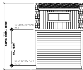
9 REAR ELEVATION SCALE: 1/4" = 1'-0"
