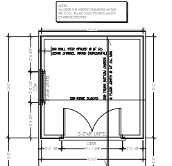
2 FLOOR PLAN SCALE: 1/4" = 1'-0"
