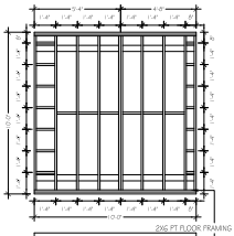
1 FLOOR FRAMING SCALE: 1/4" = 1'-0"
