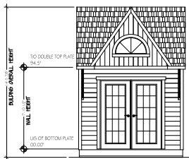
7 FRONT ELEVATION SCALE: 1/4" = 1'-0"
