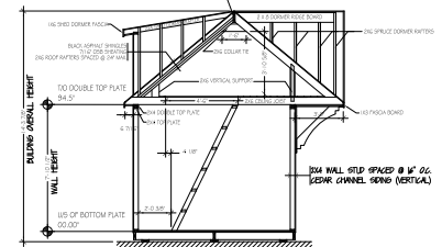
11 BUILDING SECTION SCALE: 1/4" = 1'-0"
