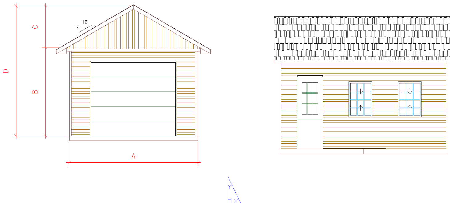
Figure 2.1a: Front and Roof Elevation (Soffit Overhang is 12")
