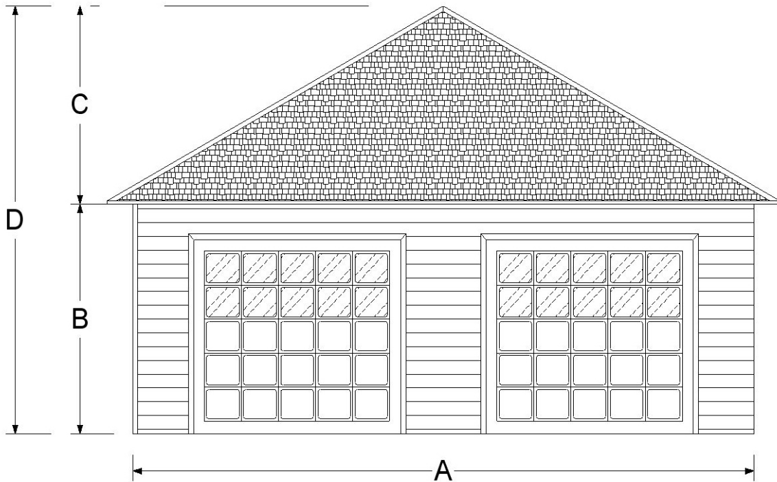
Figure 2.1a: Front Elevation
