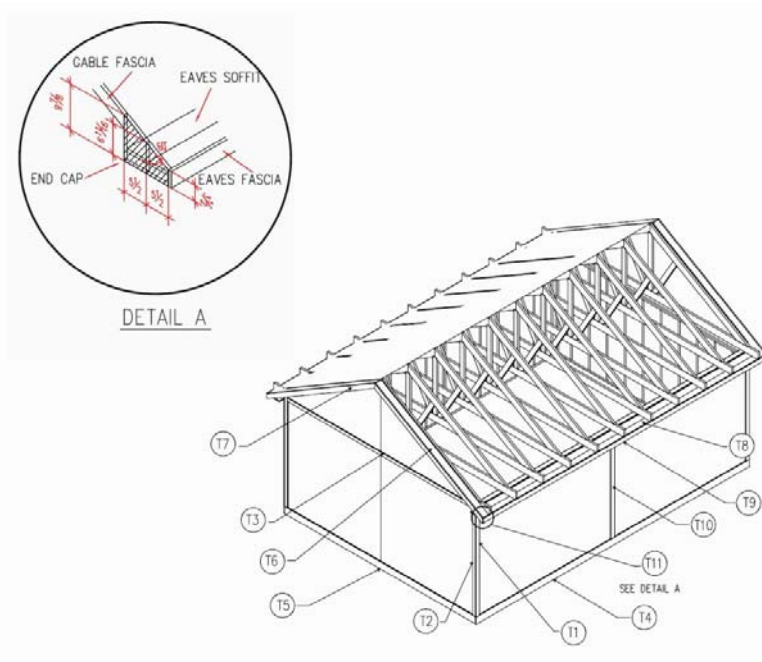
Figure 3.4a: Material Detail
