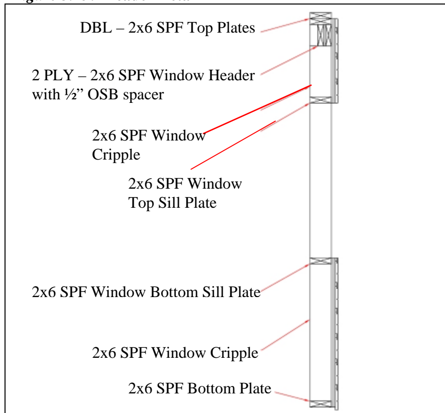
Figure 3.2b: Header Detail
